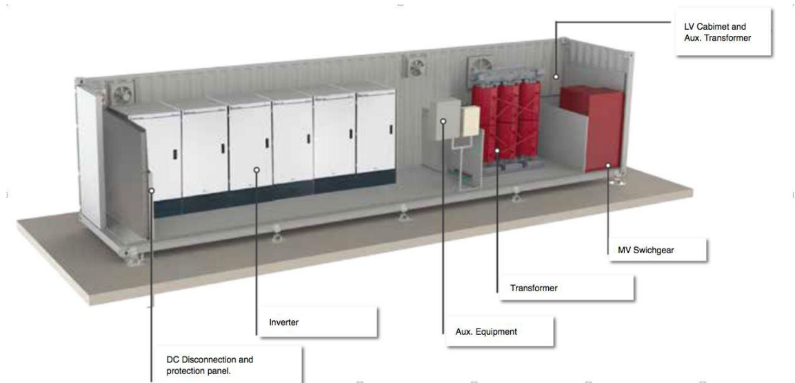
Plate 4.4 Integrated Conversion Unit
