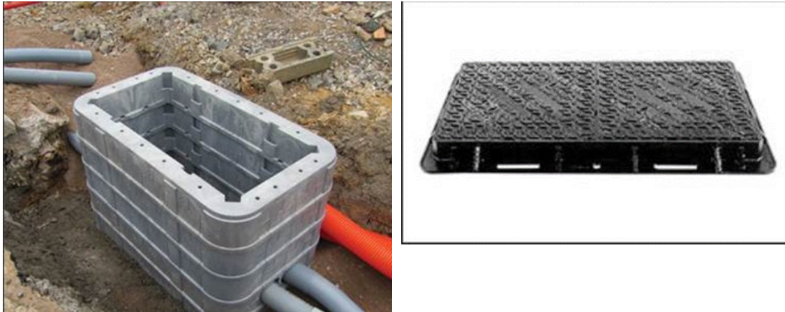
Plate 4.11 Fibre Chambers (construction and external appearance)
